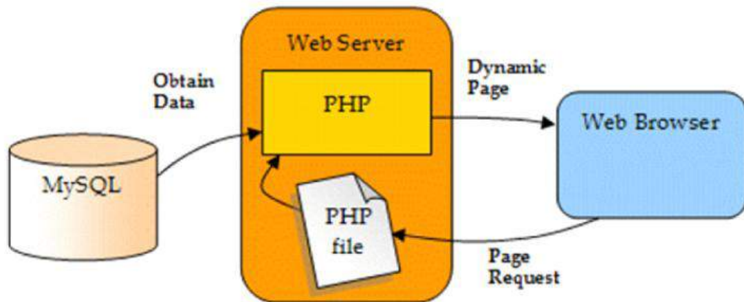
Fig. 10.5: Interactions between Browser, PHP and Database
