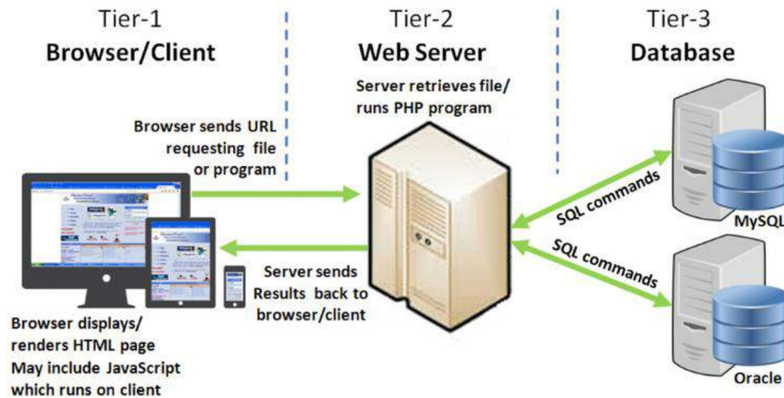
Fig 10.3: Three Tier Architecture
