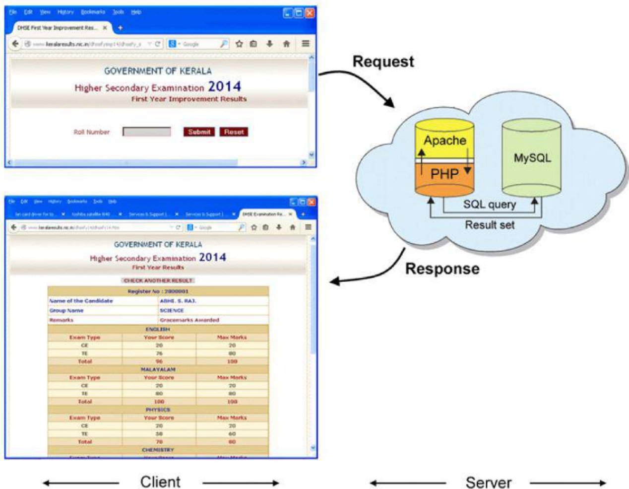
Fig : 10.4 Information flow between client and server
