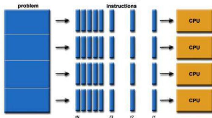
Fig.11.3: Parallel processing
