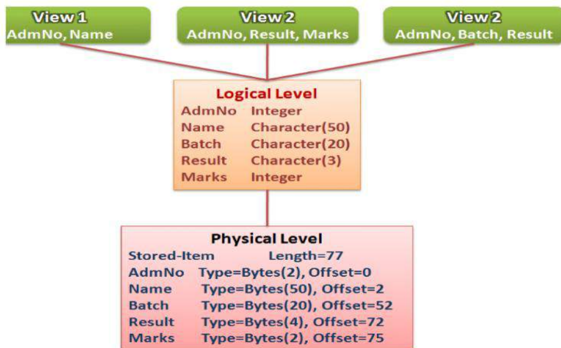
Fig. 8.4: Example for levels of abstraction
