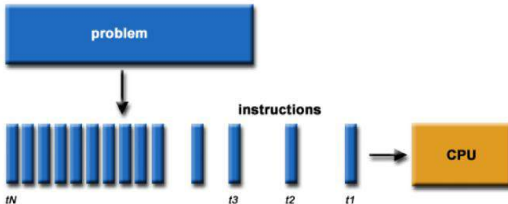
Fig. 11.2: Serial processing
