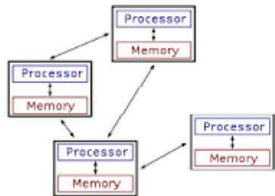
Fig. 11.1: Distributed computing
