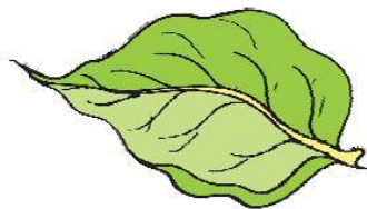
a leaf
