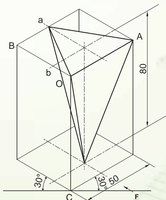
ISOMETRIC PROJECTION
