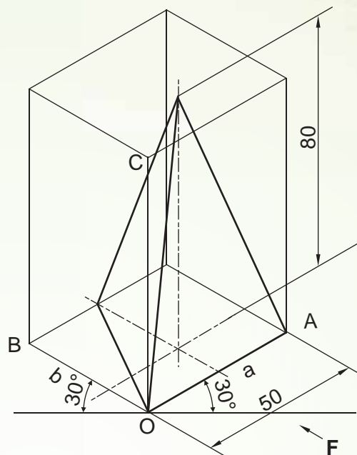
ISOMETRIC PROJECTION
