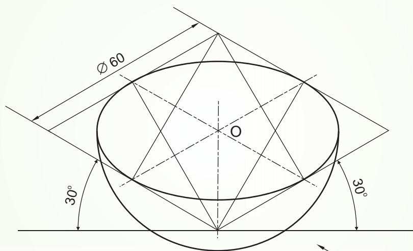
ISOMETRIC PROJECTION
