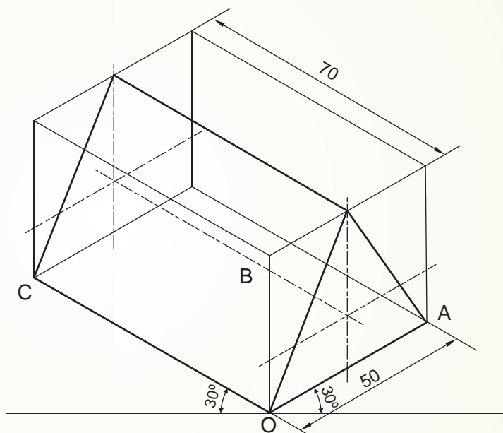
ISOMETRIC PROJECTION
