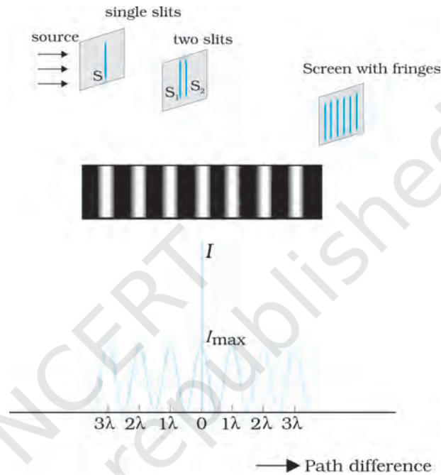
FIGURE 10.14 Photograph and the graph of the intensity distribution in Young's double-slit experiment.
